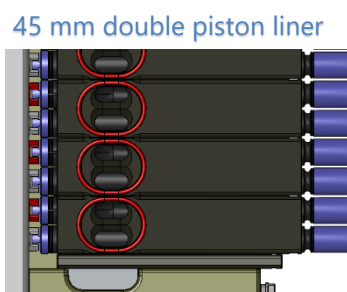
Example of a hybrid solution Left 45 mm liner – right 90 mm NI liner
